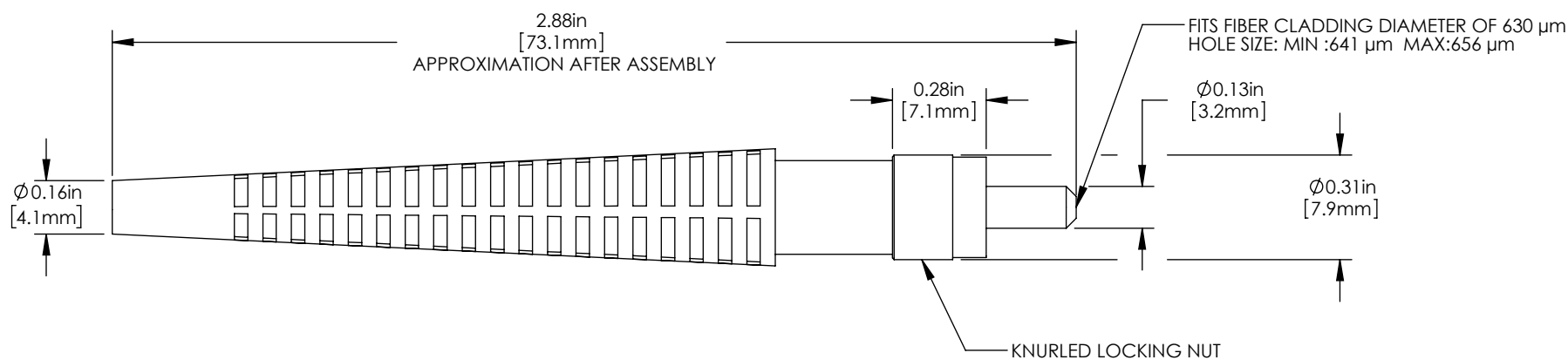
ASSEMBLED VIEW
