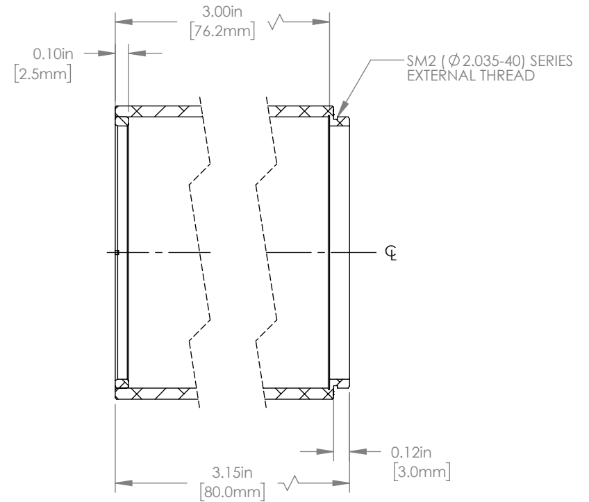
SECTION X-X
